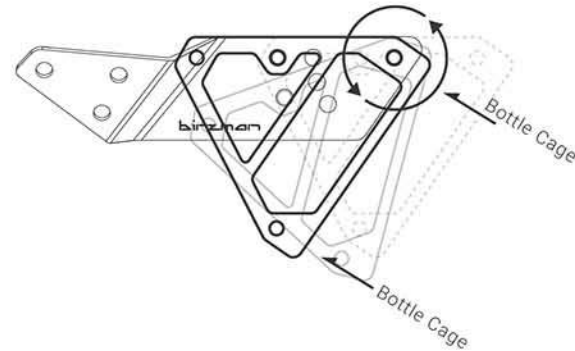
Optional Uncage Repair Kit attachment at rear end. (BM17-UNCAGE-RP-KIT)
